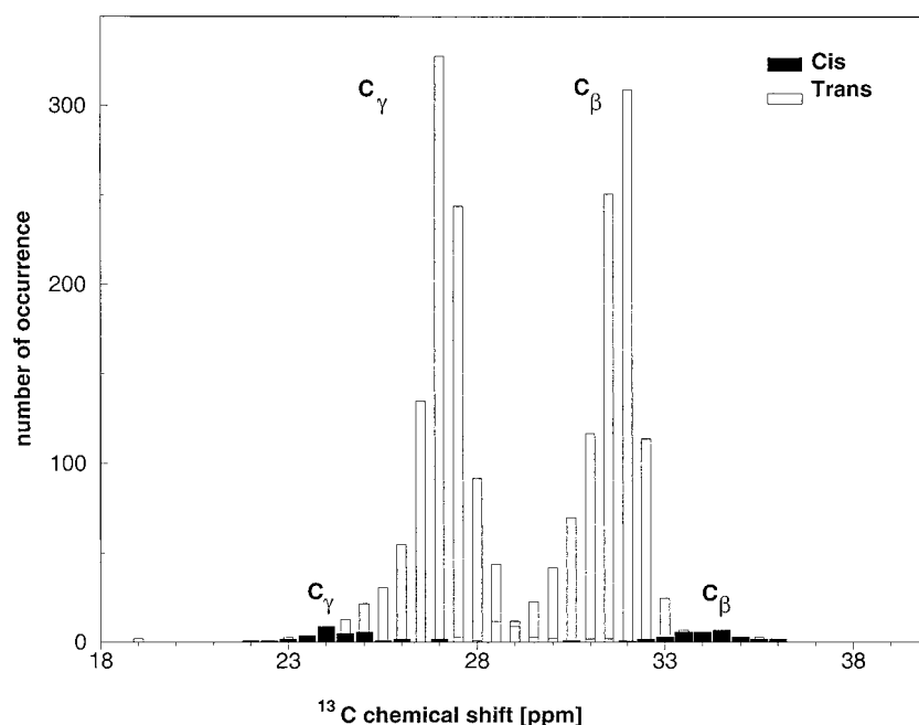
Figure 1. Number of occurrence of Xaa-Pro peptide bond conformations as a function of the proline ^{13}\text{C}^\beta and ^{13}\text{C}^\gamma chemical shifts, plotted in 0.5 ppm intervals. The statistical values are listed in Table 1.
