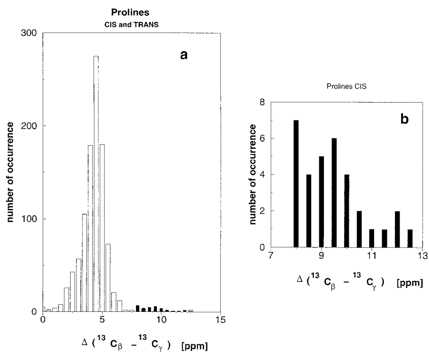
Figure 3. Number of occurrence of the Xaa-Pro peptide bond conformation as a function of the chemical shift difference \Delta_{\beta\gamma} ( \Delta_{\beta\gamma} = \delta[^{13}\text{C}^\beta] - \delta[^{13}\text{C}^\gamma] ), plotted in 0.5 ppm intervals. The statistical values are listed in Table 2. (a) both cis and trans conformation are shown; (b) only the cis conformation is shown on a larger scale.
