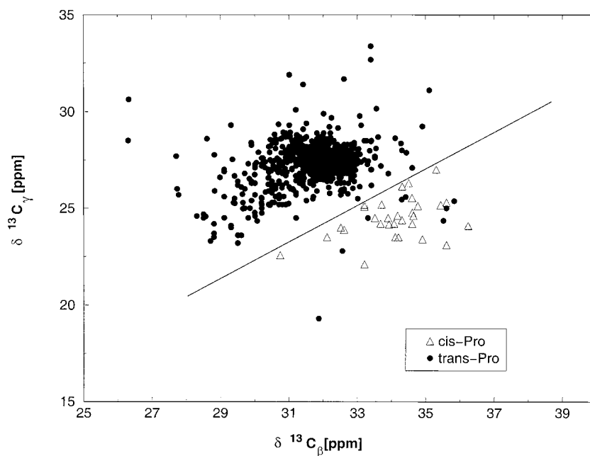
Figure 2. Two-dimensional plot of ^{13}\text{C}^\beta and ^{13}\text{C}^\gamma chemical shifts as a function of the Xaa-Pro peptide bond conformation. The solid line shows approximately the border between the two clusters of cis and trans proline conformations. Eight data points resulting from trans Xaa-Pro peptide bonds occur among the region of cis Xaa-Pro peptide bonds. It is possible that these reflect incorrectly assigned peptide bond conformations.
